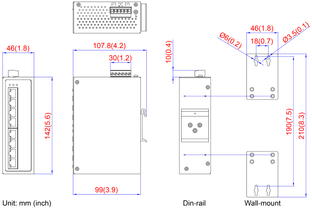
Figure 2.1: Physical Dimensions
