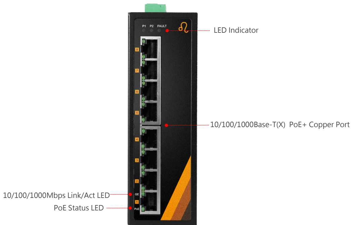
Figure 2.2: The Front Panel
