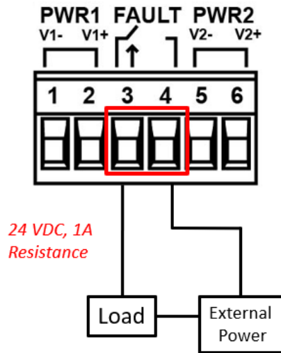
Figure 2.6: Wiring the Fault Alarm Contact
