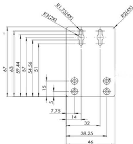
Figure 3.5: Wall Mounting Bracket Dimensions
