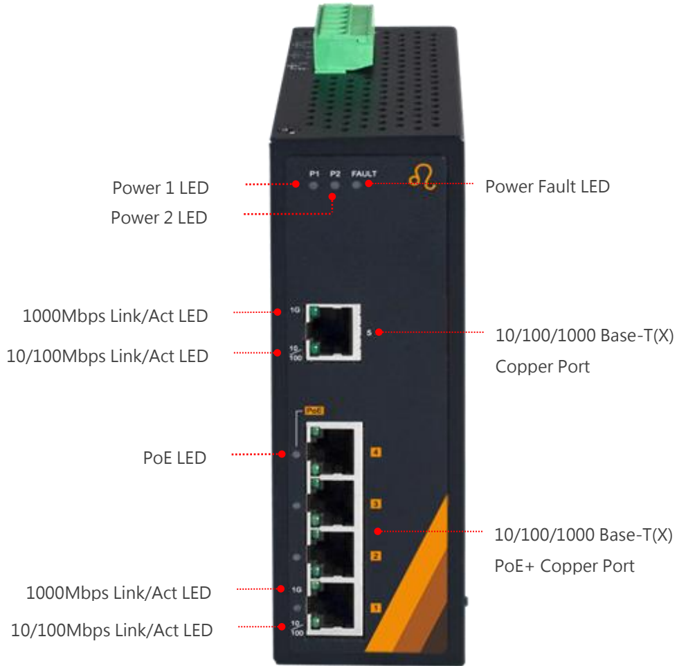
Figure 2.2: The Front Panel
