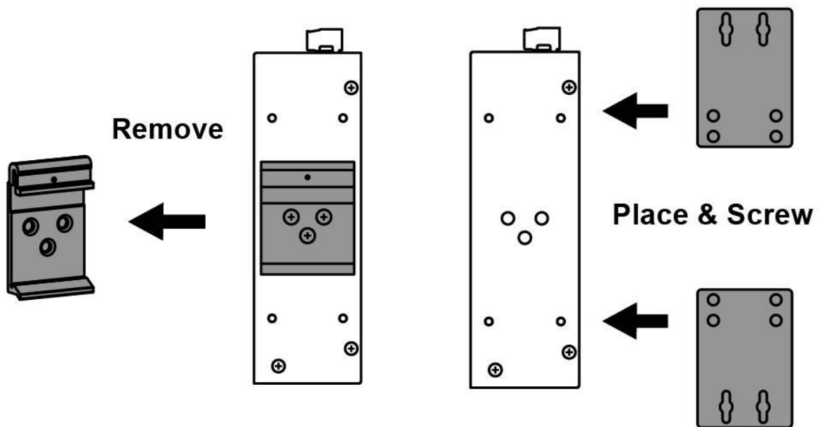
Figure 3.4: Remove DIN-Rail Bracket from the Switch and Install the Wall Mount Bracket
