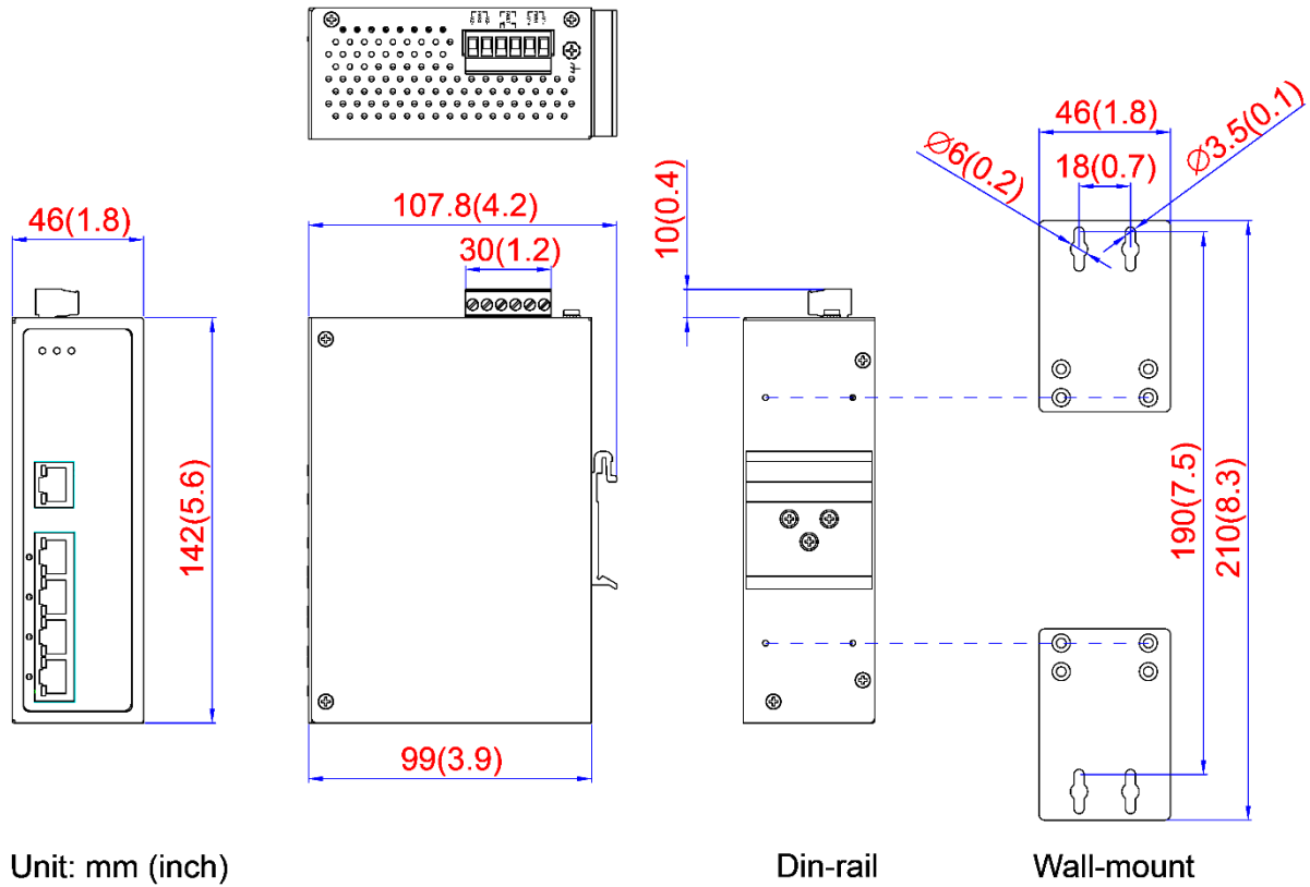
Figure 2.1: Physical Dimensions
