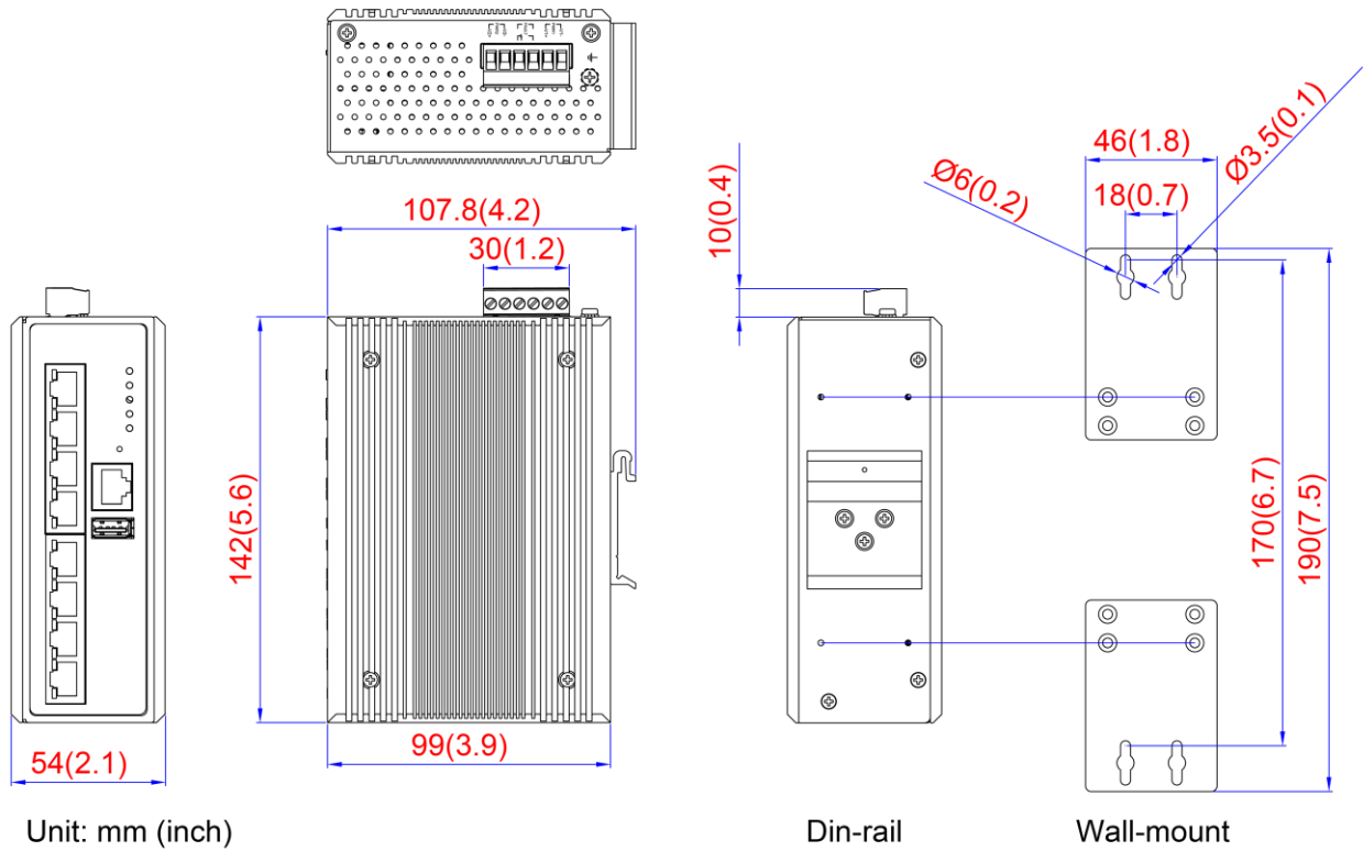
Figure 2.1: Physical Dimensions
