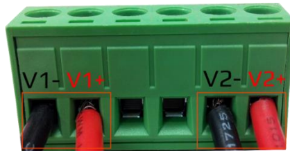
Figure 2.4: Power Terminal Block
