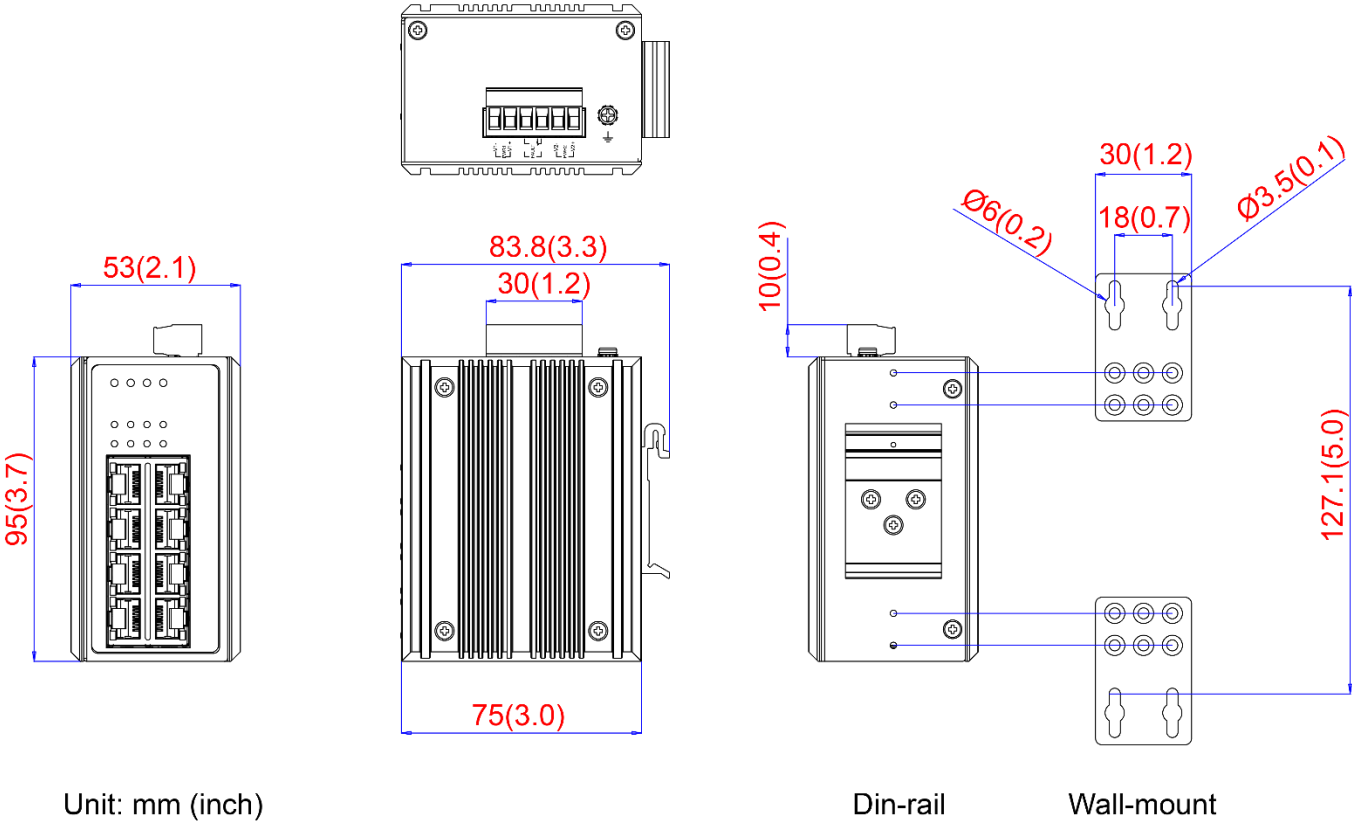
Figure 2.1: Physical Dimensions
