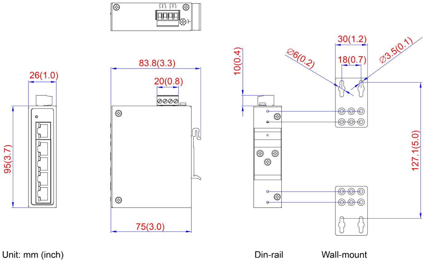
Figure 2.1: Physical Dimensions
